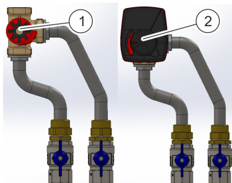
Fig. 19: Two-zone stratifier
