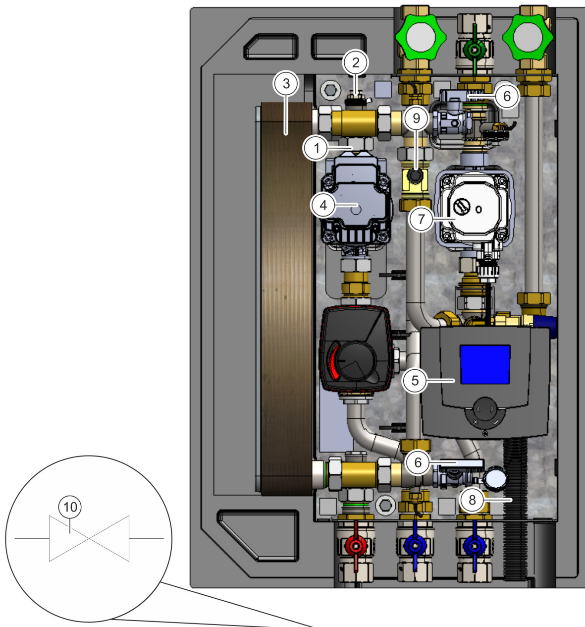
Fig. 7: Position of the components and options
