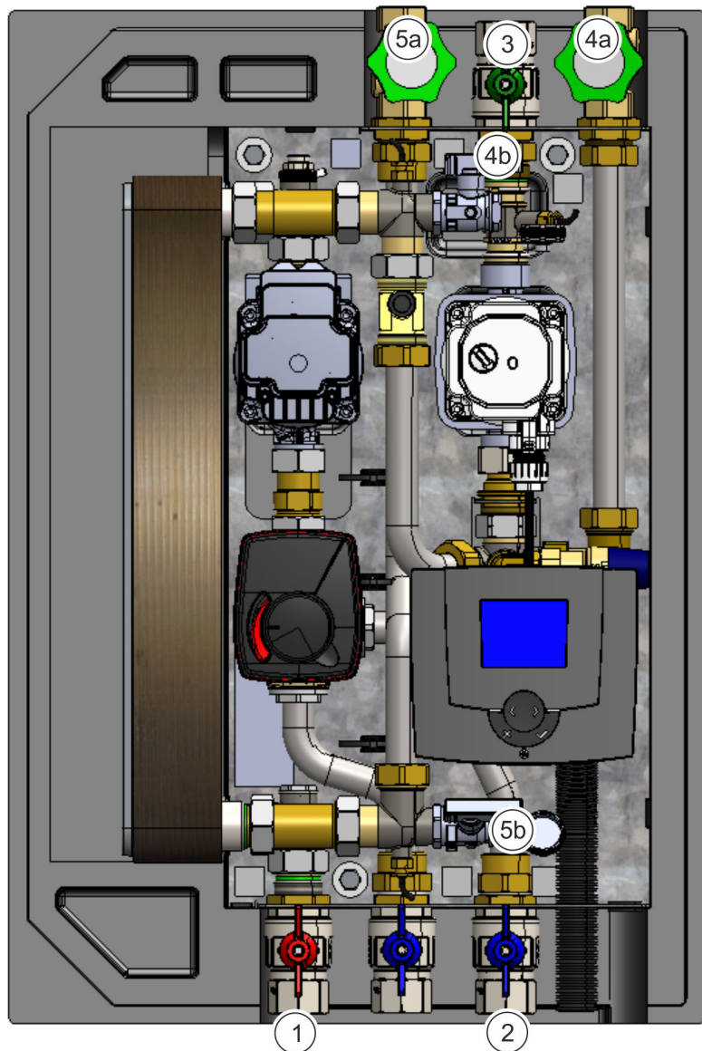
Fig. 26: Filling the fresh hot water station
