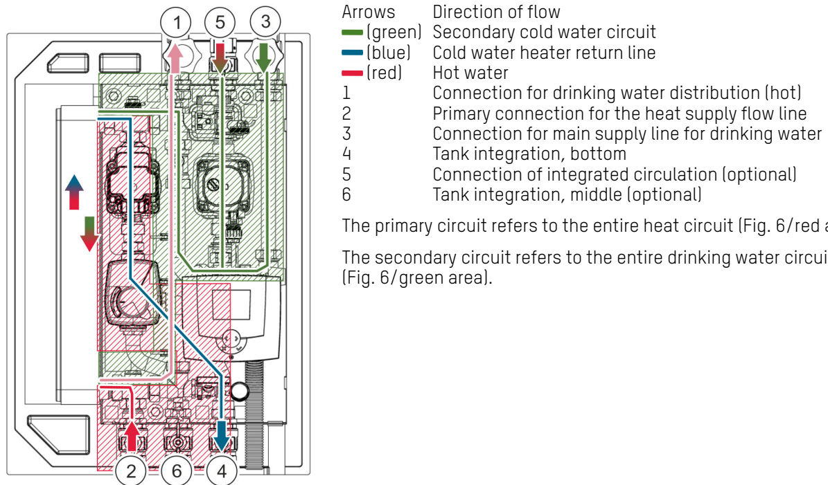
Fig. 6: Schematic overview of the lines
