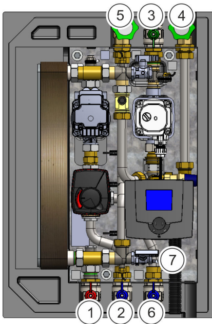
Fig. 22: Connecting cocks
