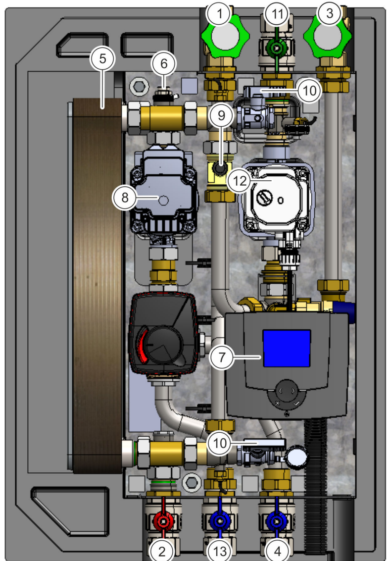
Fig. 1: Fresh hot water station
